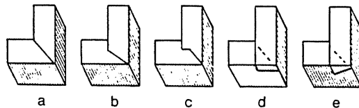
Fig. 1. OK miter joints (a) simple; (b) shoulder; (c) double shoulder; (d) miter housing; (e) dovetail miter housing.
